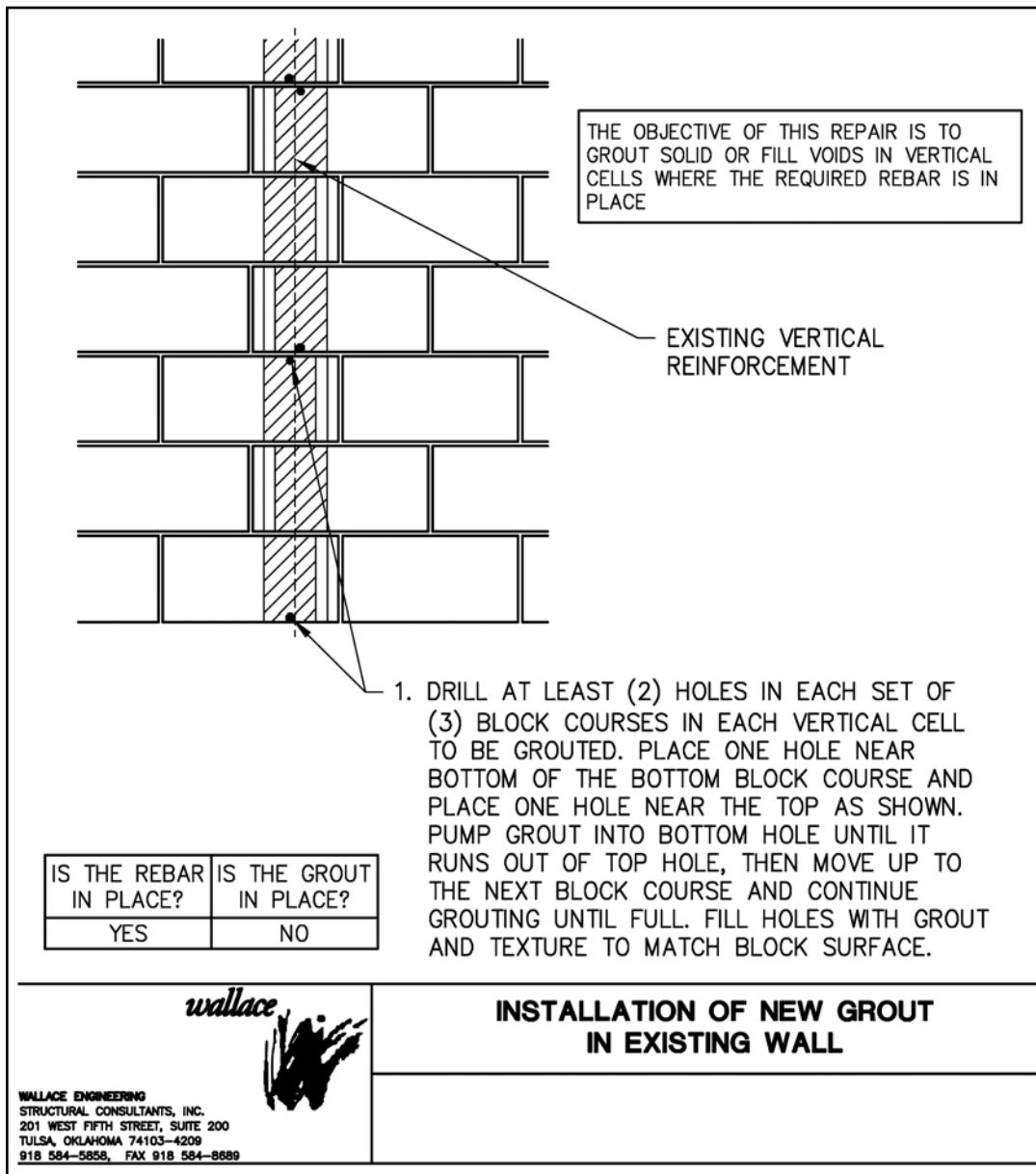
Figure 5: Sample Repair Detail for a CMU Wall with Vertical Discontinuities
